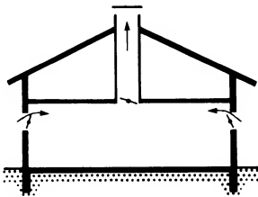
2 Stack ventilation
